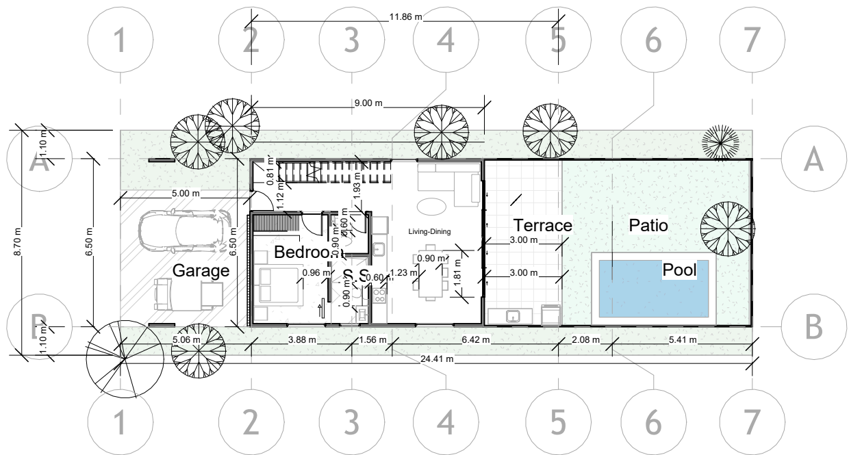
1 MODEL N1 6.5 Width B 1 : 200
